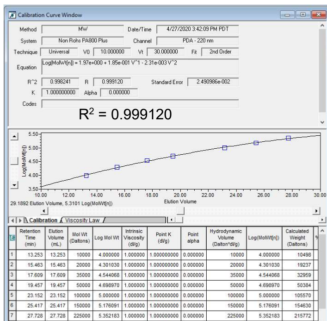
Figure 3: Calibration curve generated by the Empower software.
